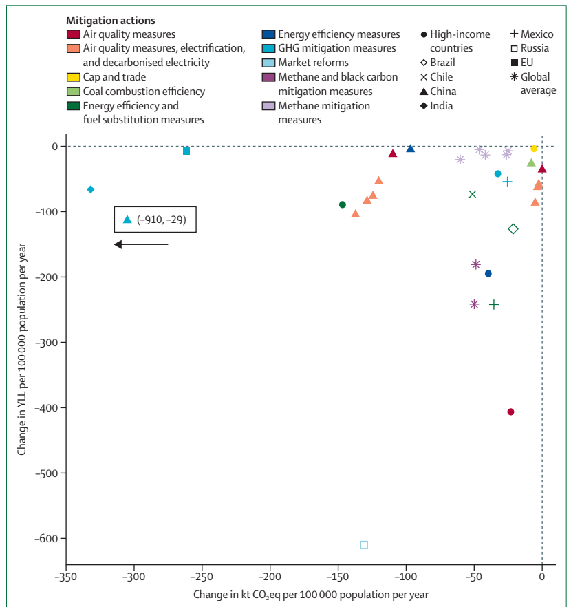
Figure 8: Climate and human health impacts of mitigation action from multisectoral actions The different-shaped points represent different types of country: circles represent high-income countries; open diamonds represent Brazil; crosses represent Chile; triangles represent China; pluses represent Mexico; open squares represent Russia; stars represent global averages; diamonds represent India; and closed squares represent the EU. Note differences in the vertical scale for changes in YLL when making comparisons between sectors. CO 2 eq=CO 2 equivalent. GHG=greenhouse gas. kt=kilotonnes. YLL=years of life lost.
